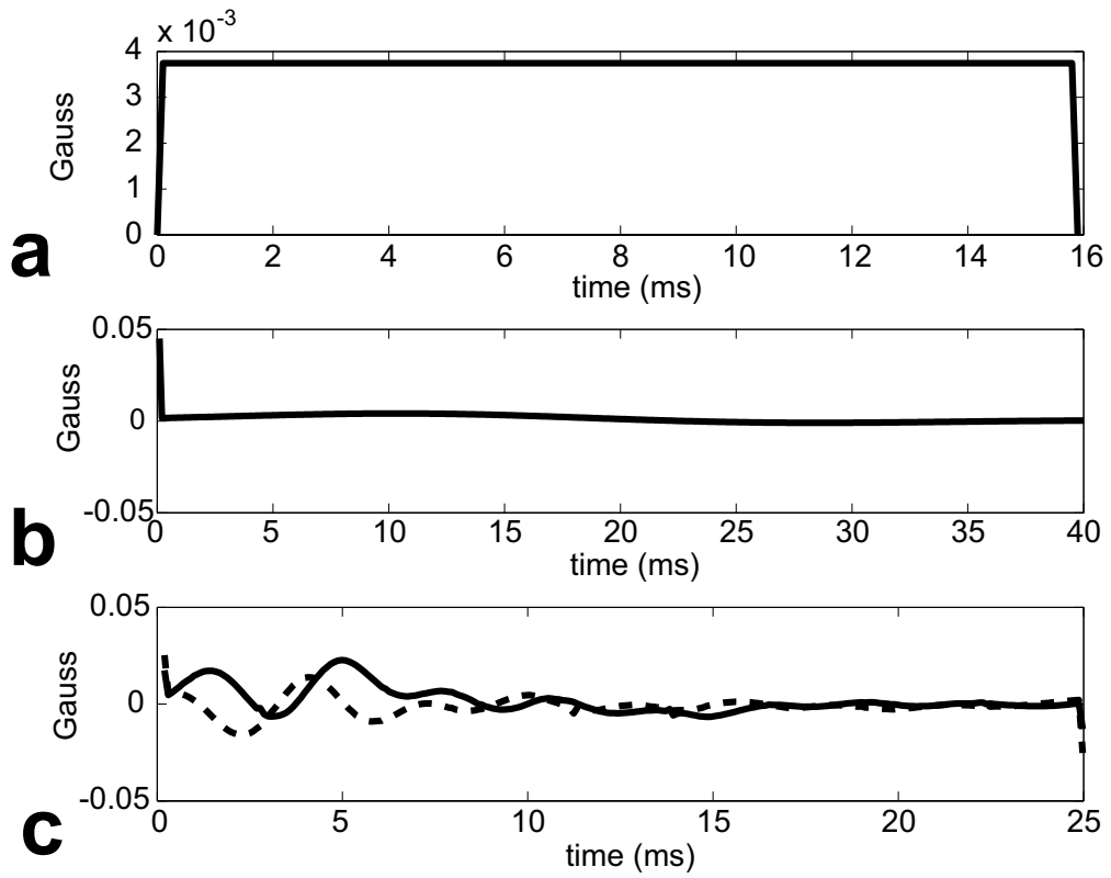
Figure 3: Long- T_2 suppression pulses. (a) 16 ms rectangular suppression pulse. (b) 40 ms TBW = 2.4 single-band suppression pulse. (c) 25 ms dual-band suppression pulse with 80 Hz water suppression bandwidth and 140 Hz suppression centered at -255 Hz for fat suppression - both real (solid line) and imaginary (dashed line) components are shown.
