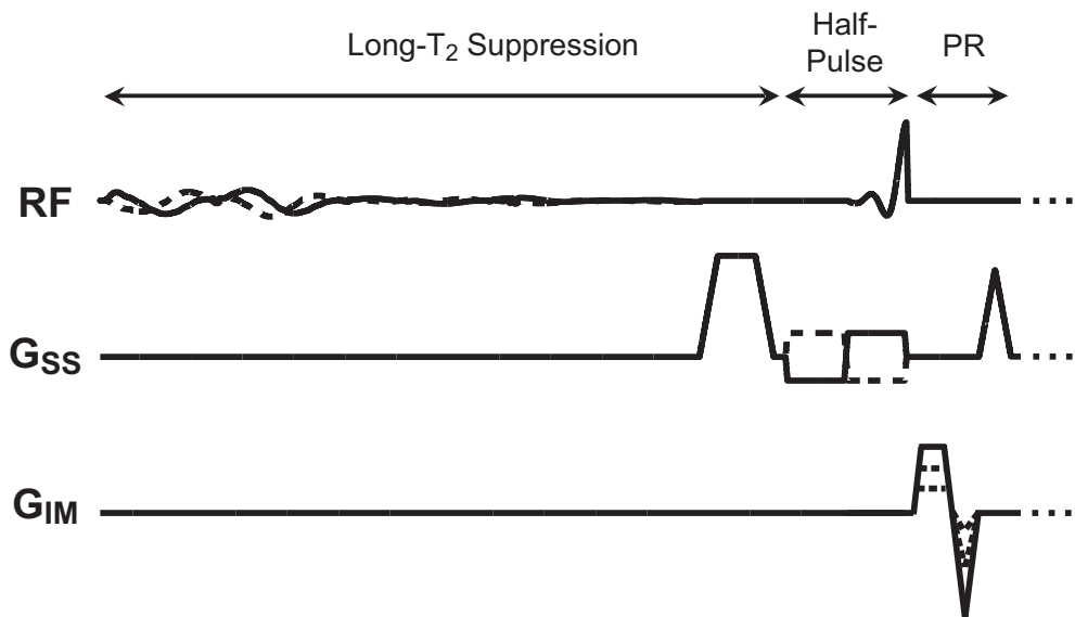
Figure 4: 2D UTE imaging sequence. The long- T_2 suppression pulse along with a dephasing gradient is played out before the half-pulse excitation. The slice-select gradient is inverted (dashed-line) between acquisitions to turn the half-pulse into a full pulse. A slice pre-phasing gradient is also included to allow for acquisition of off-isocenter slices. A projection reconstruction (PR) readout is used, and the above sequence is repeated every TR. In a 3D acquisition, the half-pulse and slice-select gradient is replaced by a hard pulse, and a twisted PR trajectory (27) is used.
