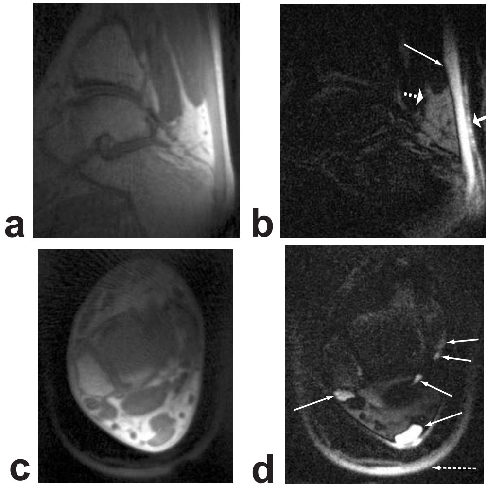
Figure 11: 3D UTE ankle images. Sagittal slice (a) without suppression and (b) with a dual-band long- T_2 suppression pulse. Axial slice (c) without suppression and (d) with suppression. The suppression significantly improves the contrast of the tendons, such as the Achilles' tendon in (b) and (d), and the peroneal, flexor hallucis longus, flexor digitorum longus, and tibialis posterior tendons in (d) (long, thin arrows). The plastic boot holding the ankle can also be seen (long, dashed arrow in (d)). Unsuppressed signal in the fat pad anterior to the Achilles' tendon (short, dashed arrow in (b)) may be due to short- T_2 components in the fat or suppression failure. Posterior to the Achilles' tendon there is also either failed suppression and/or signal from collagen in the skin (short, solid arrow in (b)).
