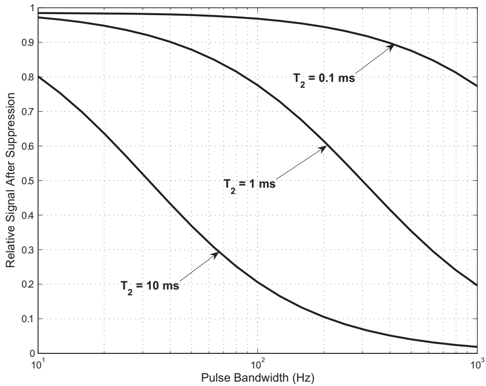
Figure 6: Simulation results for the longitudinal magnetization remaining after single-band suppression pulses of different bandwidths for various T_2 values. As the pulse bandwidth increases, the signal remaining after suppression decreases, as predicted by Eq. 8. As T_2 increases, the signal also decreases.
